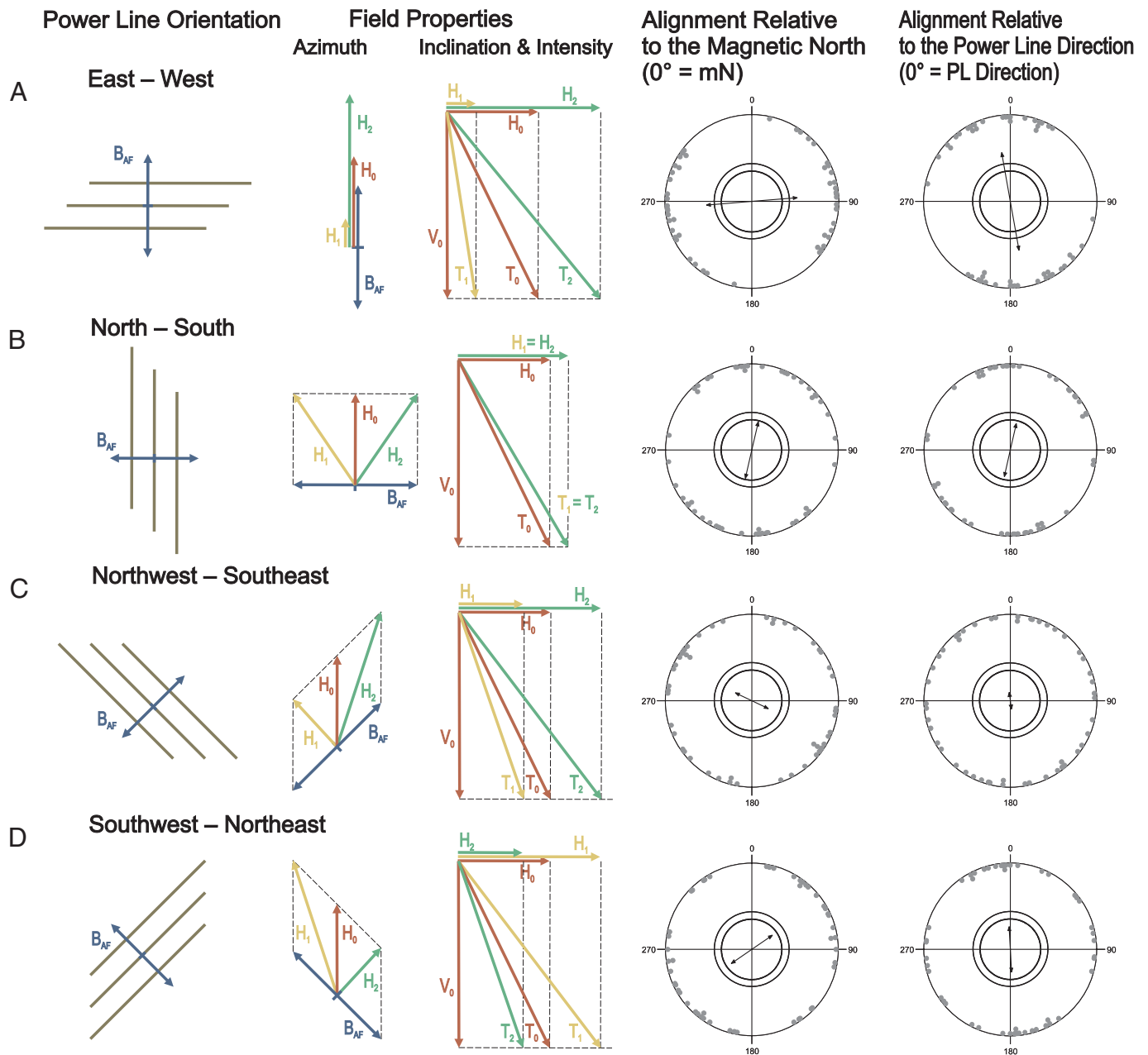
Fig. 2. Magnetic field properties and body orientation of cattle directly under power lines. Power lines trending in the ranges of 70^{\circ} – 110^{\circ} , 340^{\circ} – 20^{\circ} , 115^{\circ} – 155^{\circ} and 25^{\circ} – 65^{\circ} were classified as E-W (A), N-S (B), NW-SE (C), and NE-SW (D), respectively. The total intensity vector of the field (T) can be resolved into 2 vector components: the horizontal field intensity (H) and the vertical field intensity (V). The inclination is a vertical angle between the H (or the Earth's surface) and T. The azimuth is a horizontal angle measured clockwise between the horizontal intensity vector of the EMF ( H_0 ) and the horizontal intensity vectors of the fields resulting from summation of the AMF and EMF ( H_1 or H_2 ). B_{AF} , AMF vector; H_0 , V_0 , T_0 , vectors of the EMF; H_1 , H_2 , V_1 , V_2 , T_1 , T_2 , vectors of the fields resulting from summation of the AMF and the EMF (the actual field oscillates between H_1 and H_2 , V_1 and V_2 , and T_1 and T_2 , respectively, with a frequency of 50 Hz). Axial alignment data presented as in Fig. 1. See Tables S1 and S2 for numerical values.
